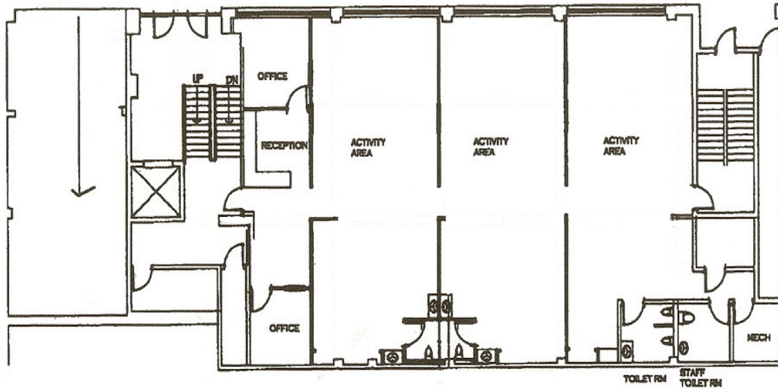
UPPER LEVEL (FIRST) FLOOR PLAN
